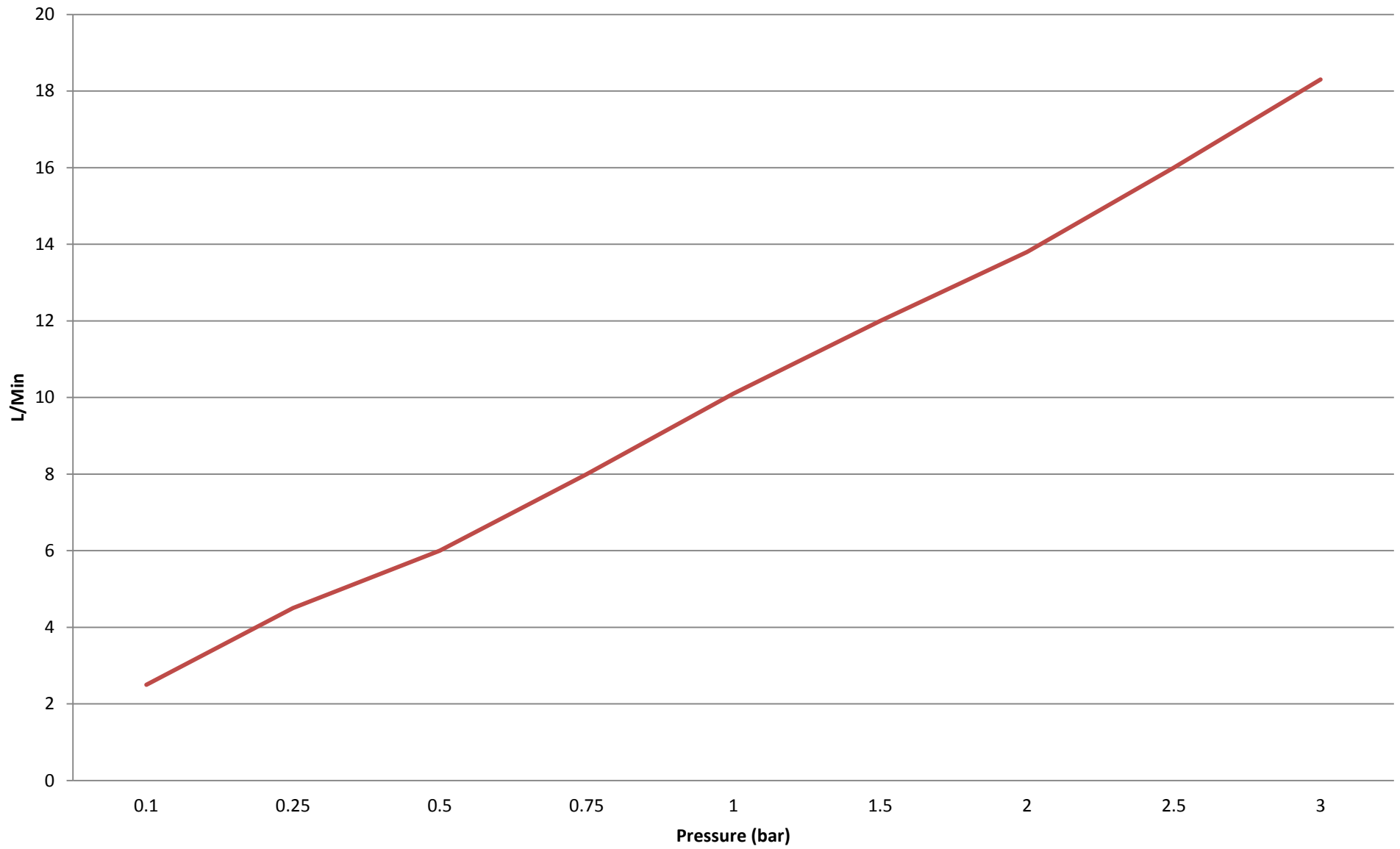
ST10010CP Flow Rate Graph
